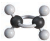
乙烯
