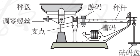
图6.1-7 案秤
